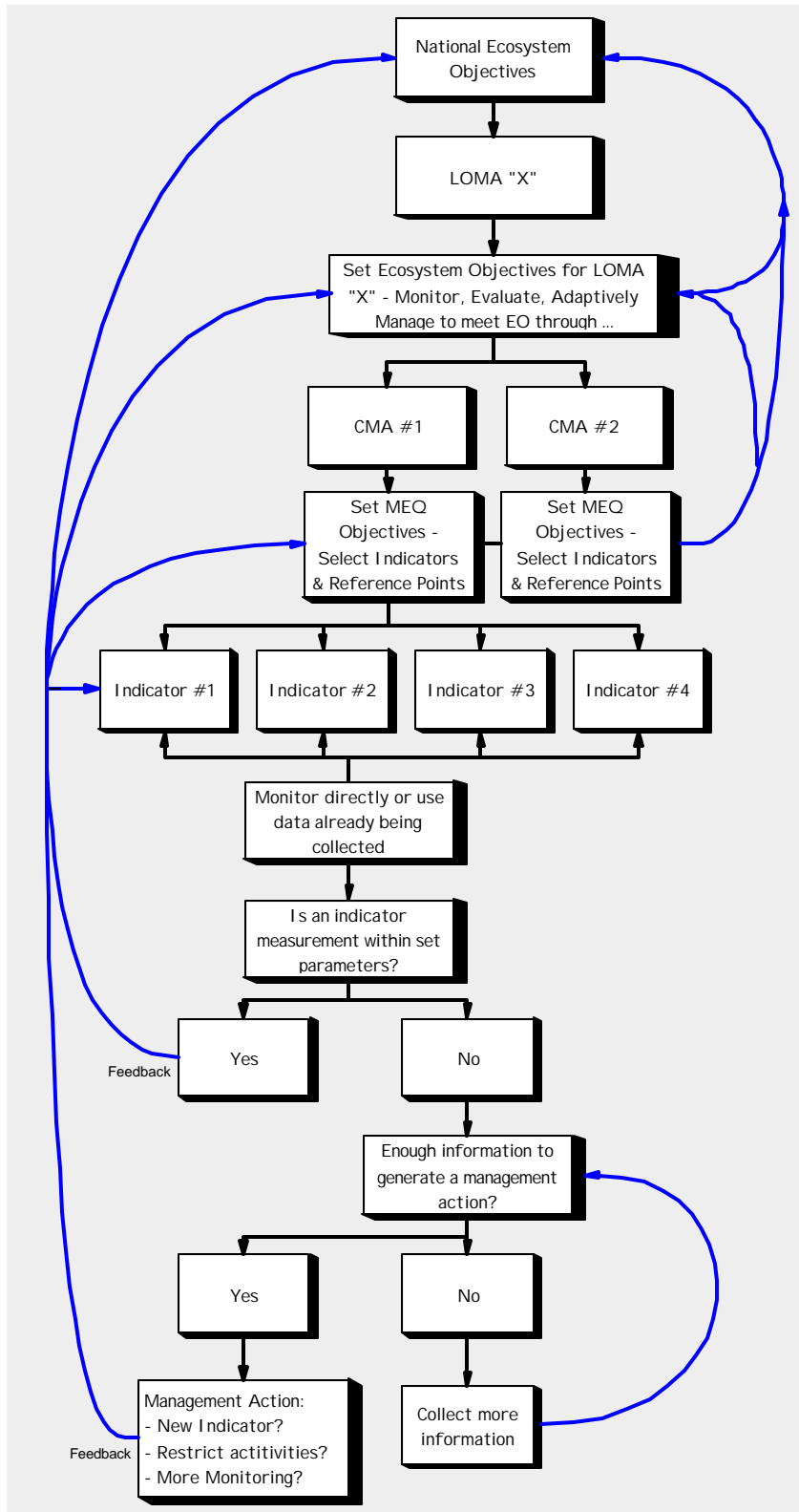
Figure 1: A flow diagram demonstrating how decisions at a CMA scale may be made with respect to the establishment of indicators and responses to indicator measures.
