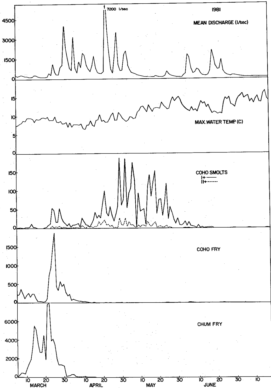
Fig. 3. Outmigration of juvenile salmonids in Carnation Creek in relation to date, water temperature and discharge, 1981.
