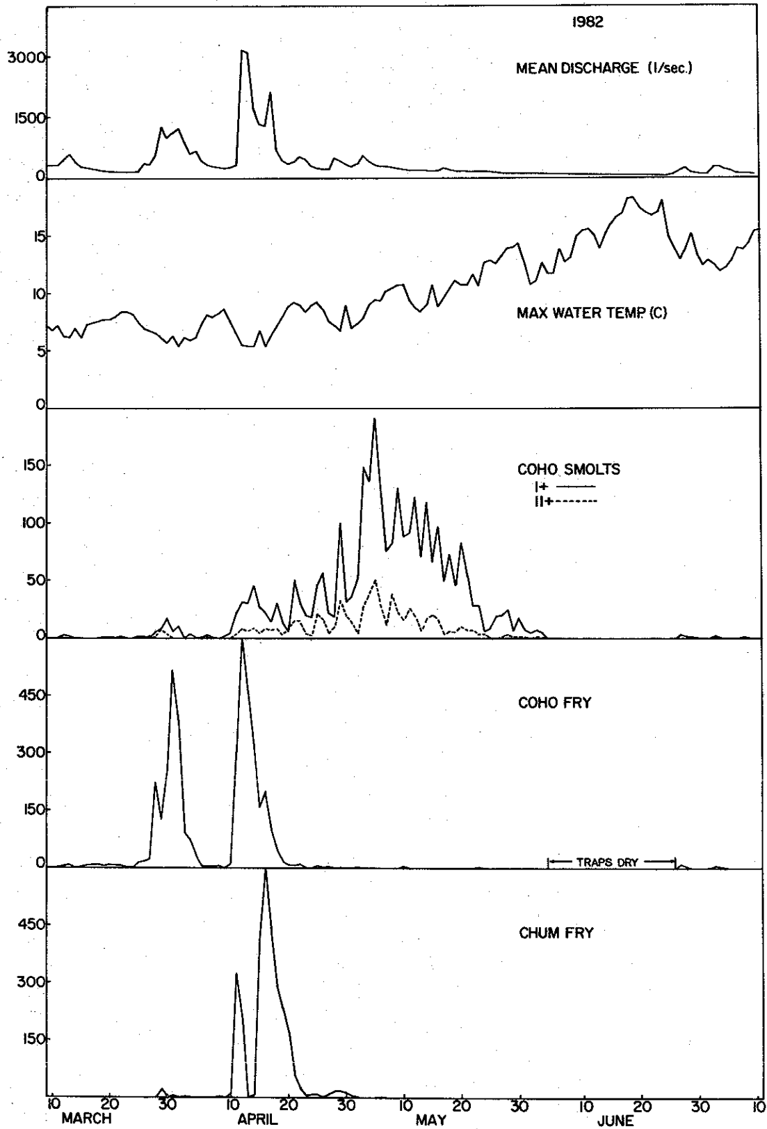
Fig. 4. Outmigration of juvenile salmonids in Carnation Creek in relation to date, water temperature and discharge, 1982.
